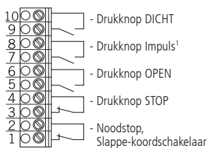
Klemmenstrip X3 (indeling)
